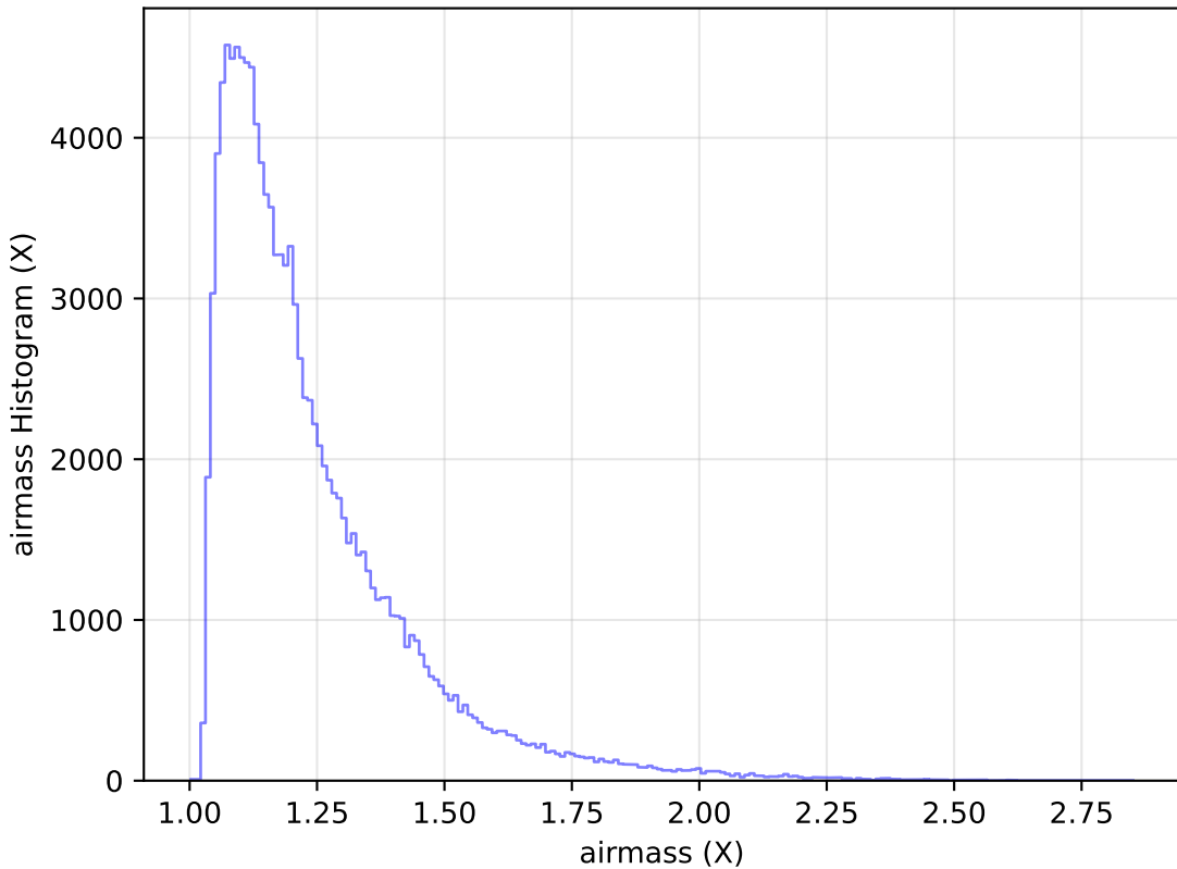
roll_pause_mjdp60_v3.4_10yrs All sky u band: airmass Histogram
