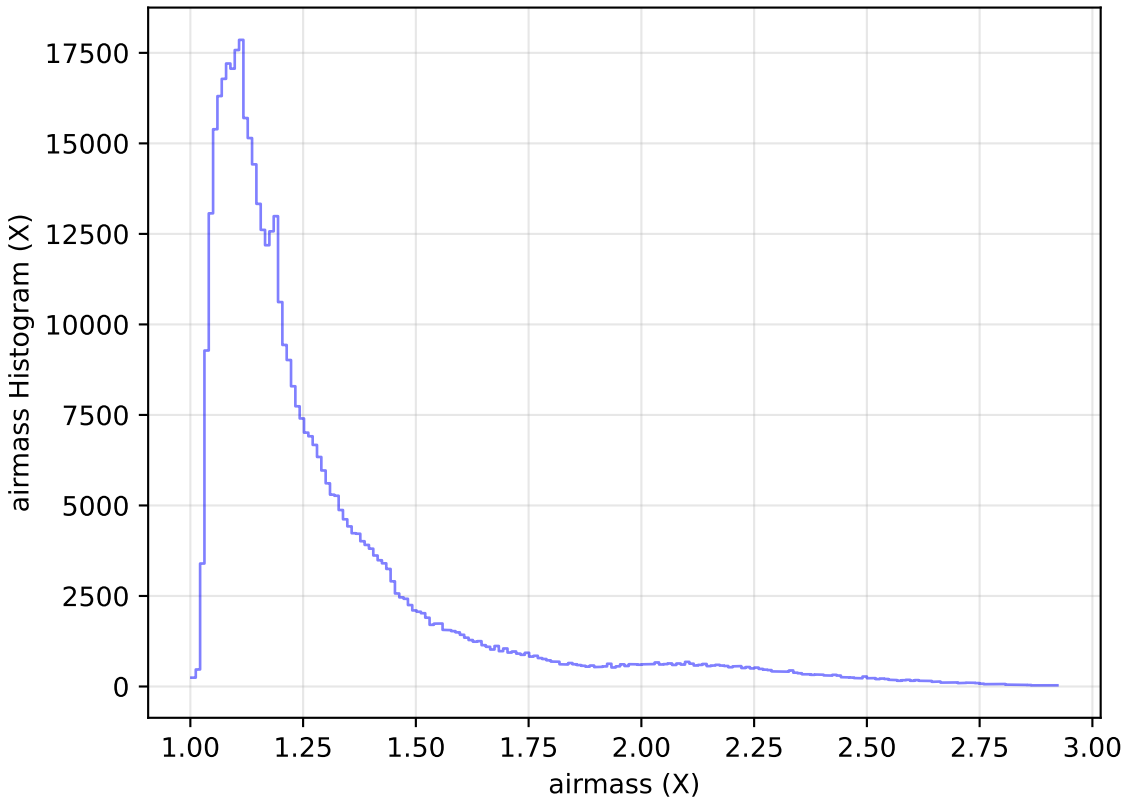
roll_pause_mjdp60_v3.4_10yrs All sky i band: airmass Histogram
