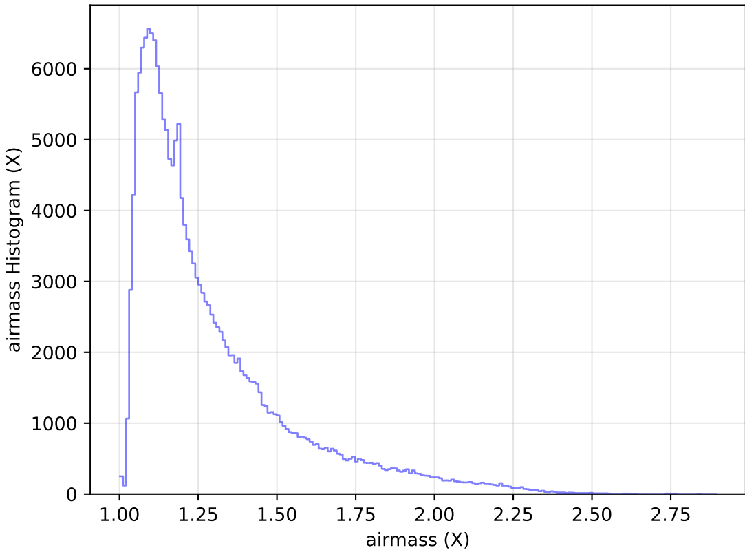
roll_pause_mjdp60_v3.4_10yrs All sky g band: airmass Histogram
