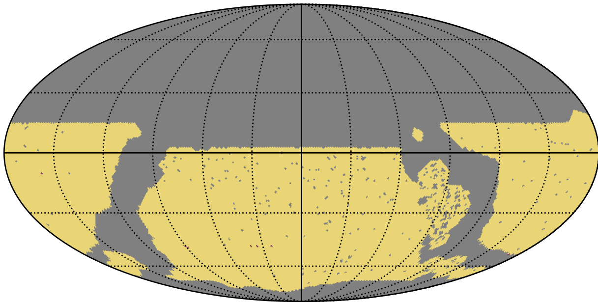
roll_pause_mjdp60_v3.4_10yrs WFD: RapidRevisits
