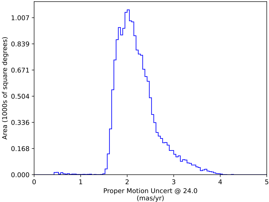
roll_pause_mjdp60_v3.4_10yrs WFD: Proper Motion Uncert @ 24.0
