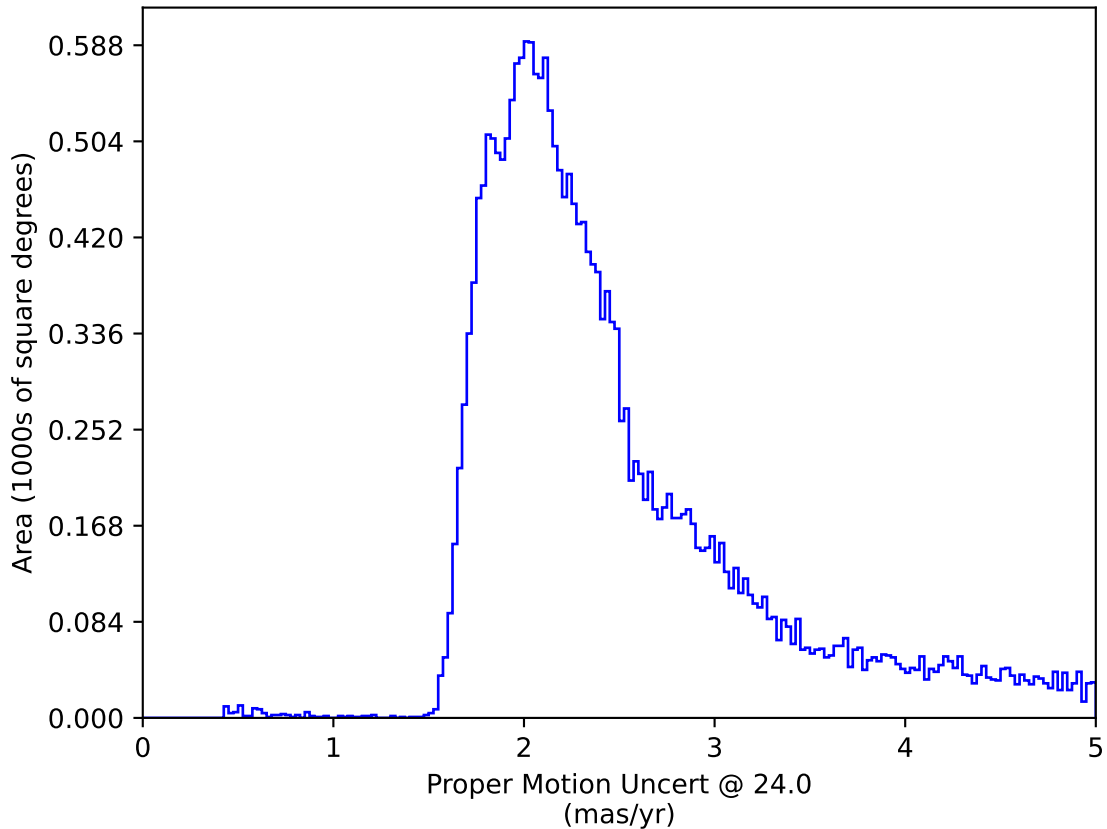
roll_pause_mjdp60_v3.4_10yrs All sky: Proper Motion Uncert @ 24.0
