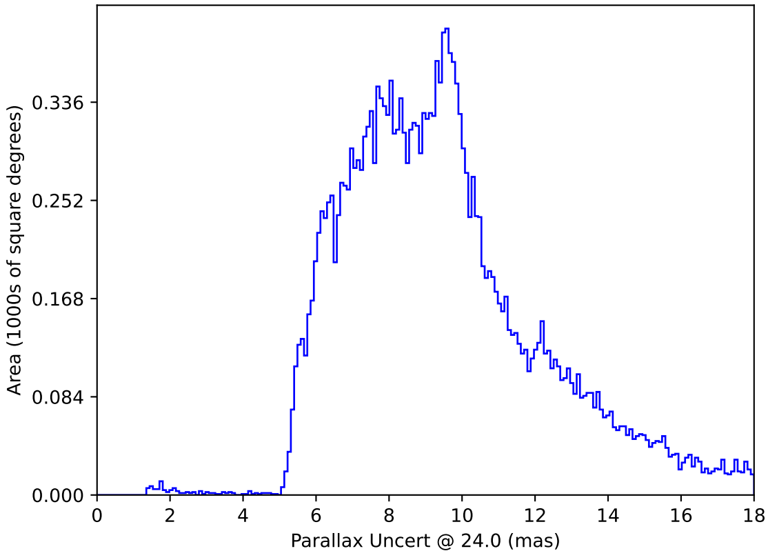
roll_pause_mjdp60_v3.4_10yrs All sky: Parallax Uncert @ 24.0
