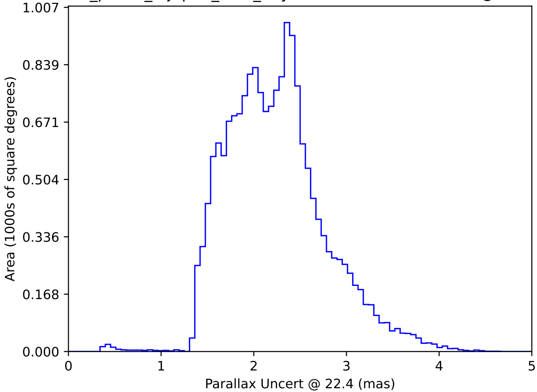
roll_pause_mjdp60_v3.4_10yrs WFD: Parallax Uncert @ 22.4
