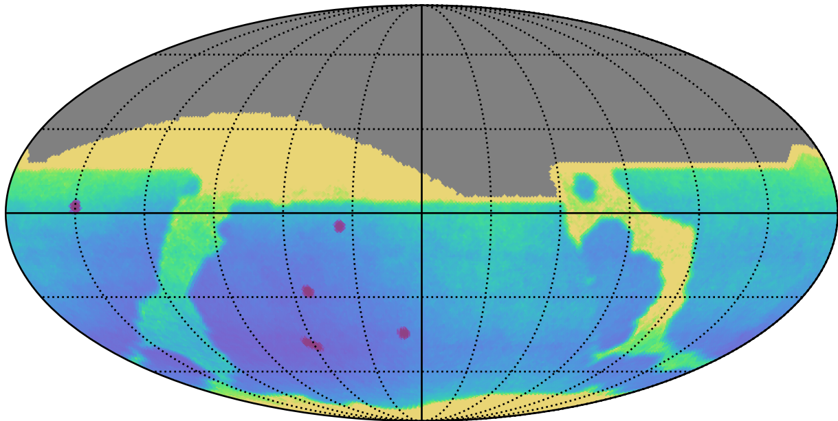
roll_pause_mjdp60_v3.4_10yrs All sky: Parallax Uncert @ 22.4
