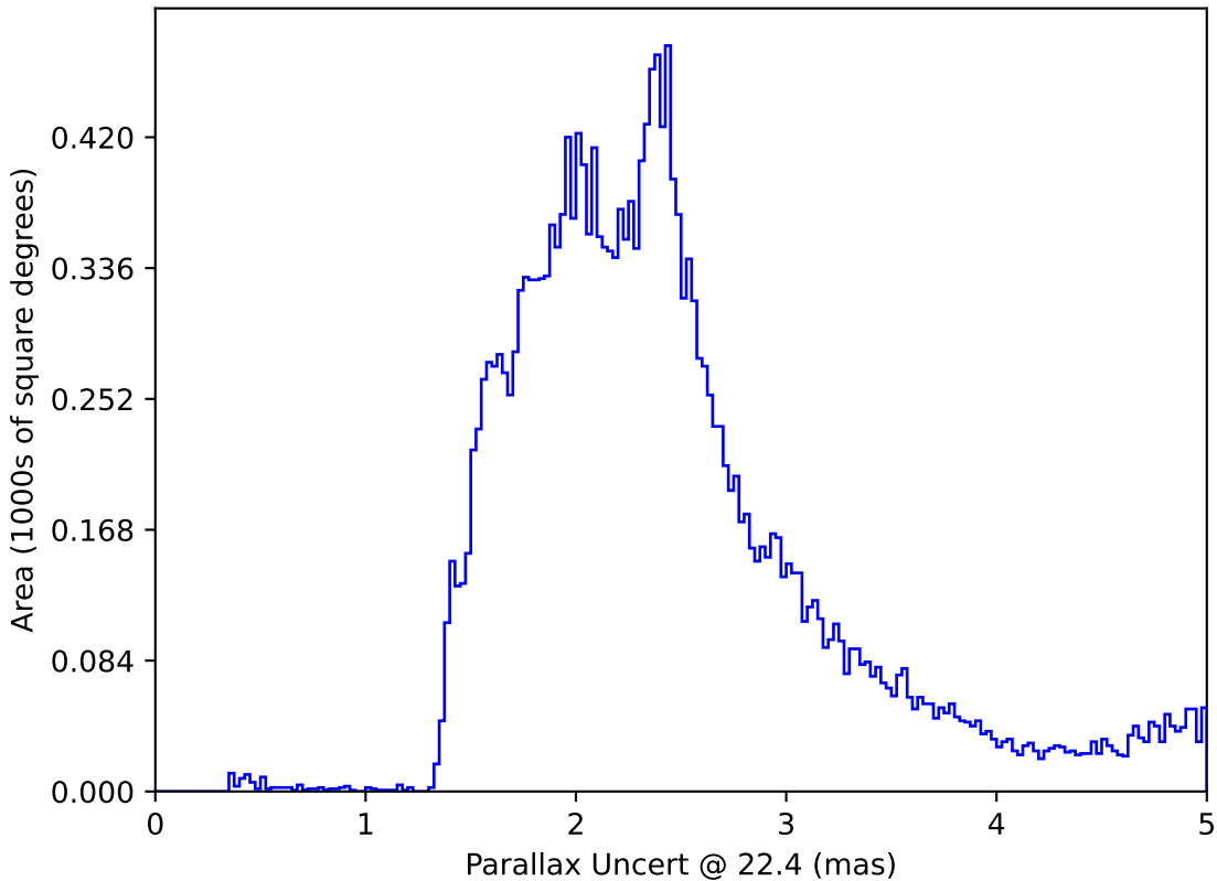
roll_pause_mjdp60_v3.4_10yrs All sky: Parallax Uncert @ 22.4
