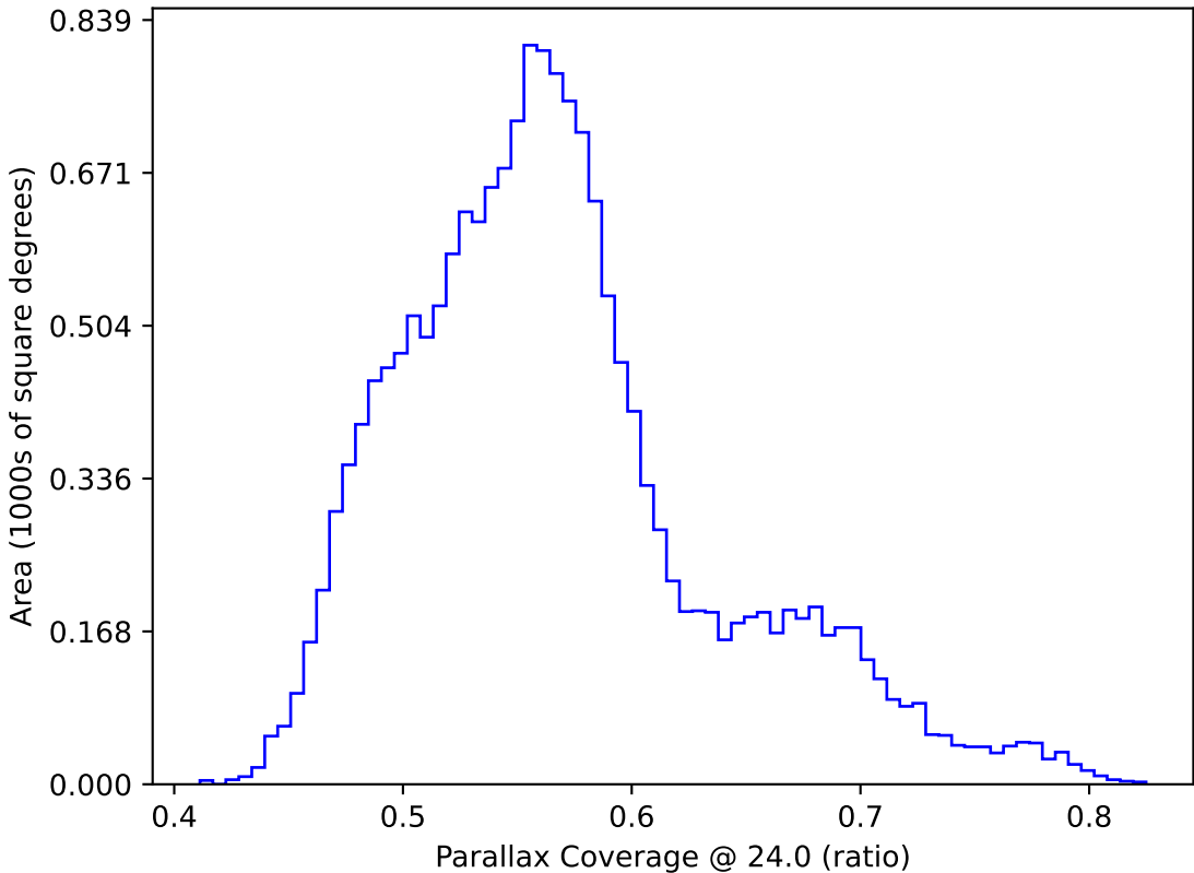
roll_pause_mjdp60_v3.4_10yrs WFD: Parallax Coverage @ 24.0
