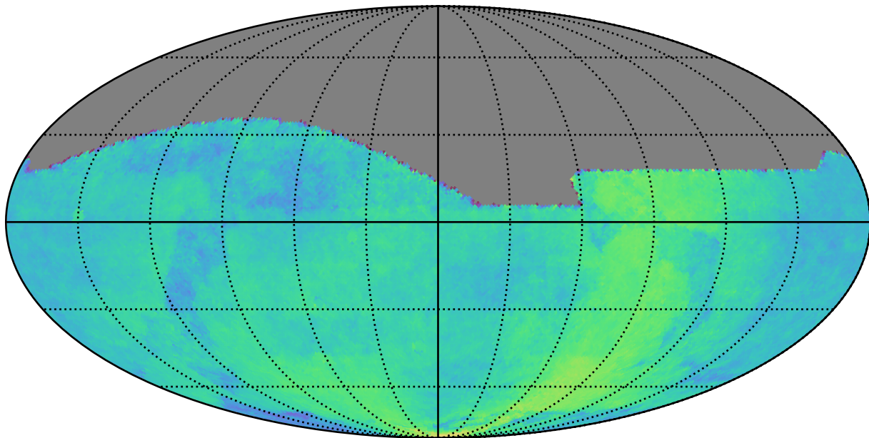
roll_pause_mjdp60_v3.4_10yrs All sky: Parallax Coverage @ 24.0
