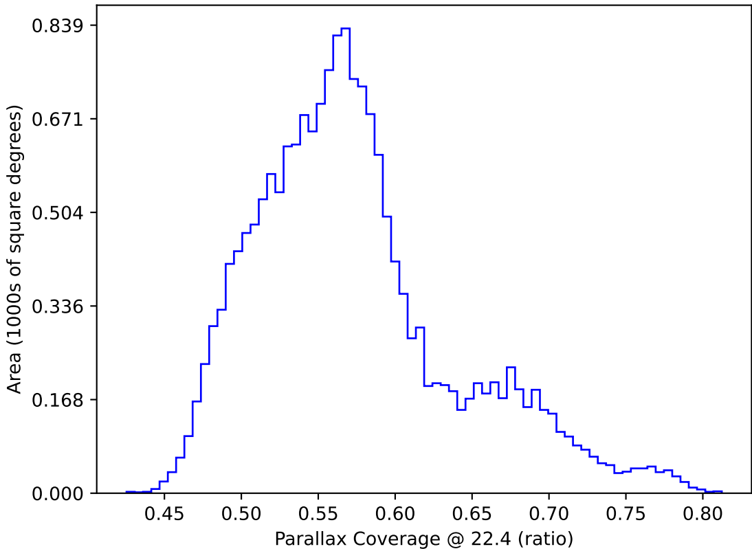
roll_pause_mjdp60_v3.4_10yrs WFD: Parallax Coverage @ 22.4
