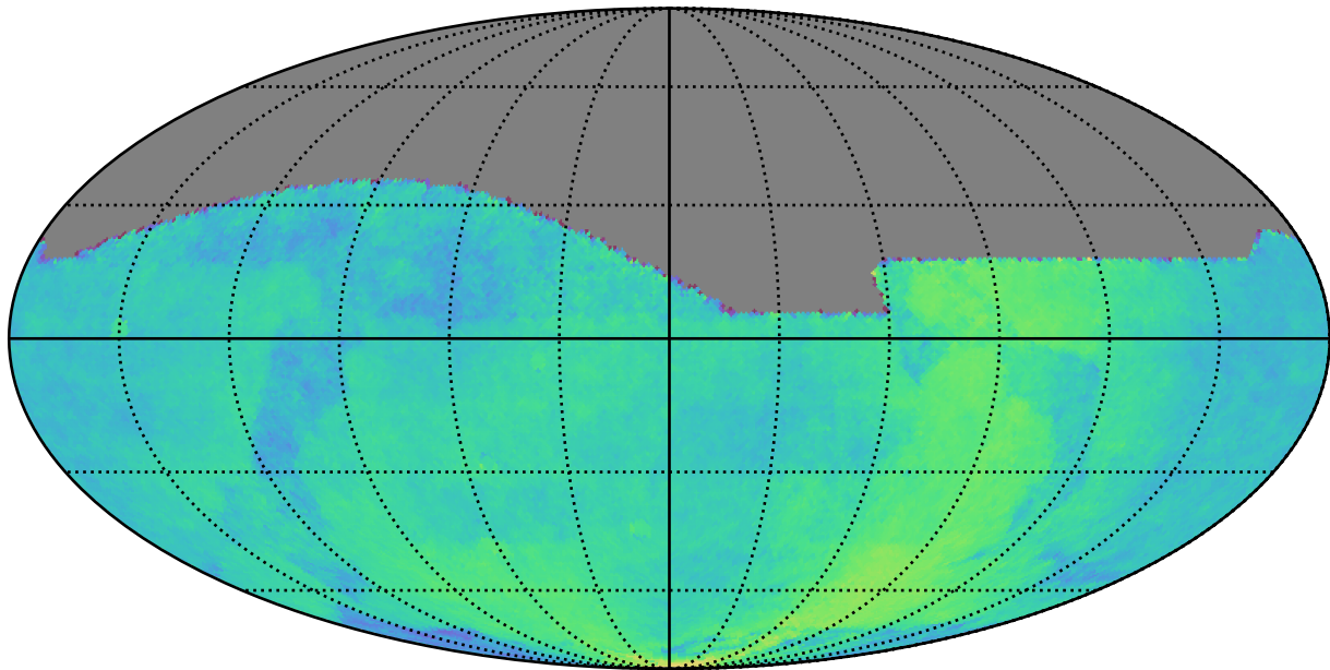
roll_pause_mjdp60_v3.4_10yrs All sky: Parallax Coverage @ 22.4
