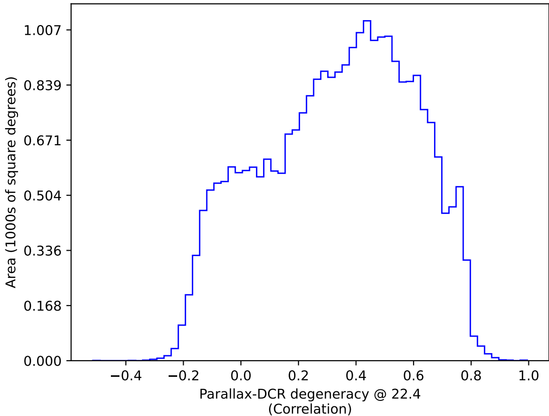
roll_pause_mjdp60_v3.4_10yrs All sky: Parallax-DCR degeneracy @ 22.4
