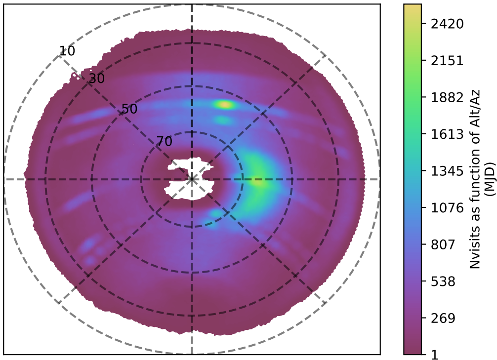
roll_pause_mjdp60_v3.4_10yrs z band: Nvisits as function of Alt/Az
