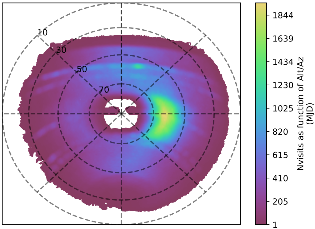
roll_pause_mjdp60_v3.4_10yrs y band: Nvisits as function of Alt/Az
