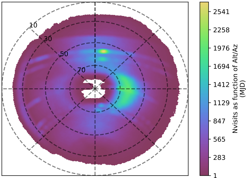
roll_pause_mjdp60_v3.4_10yrs r band: Nvisits as function of Alt/Az
