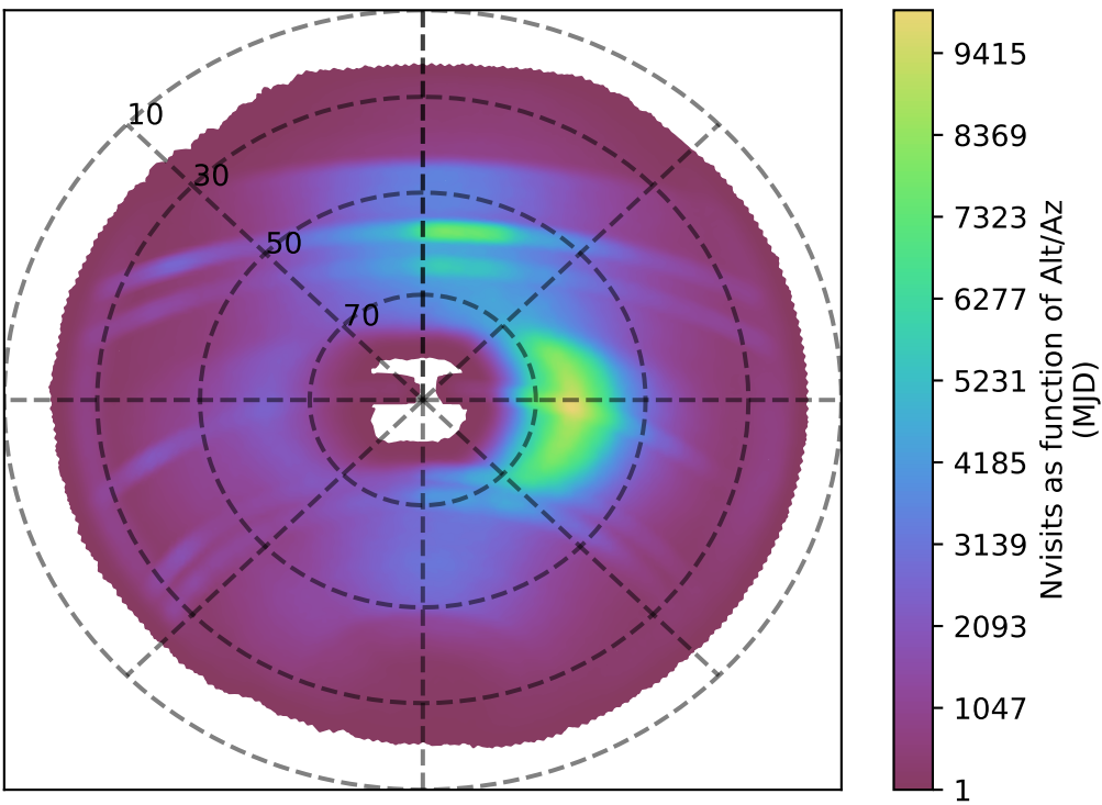
roll_pause_mjdp60_v3.4_10yrs all bands: Nvisits as function of Alt/Az
