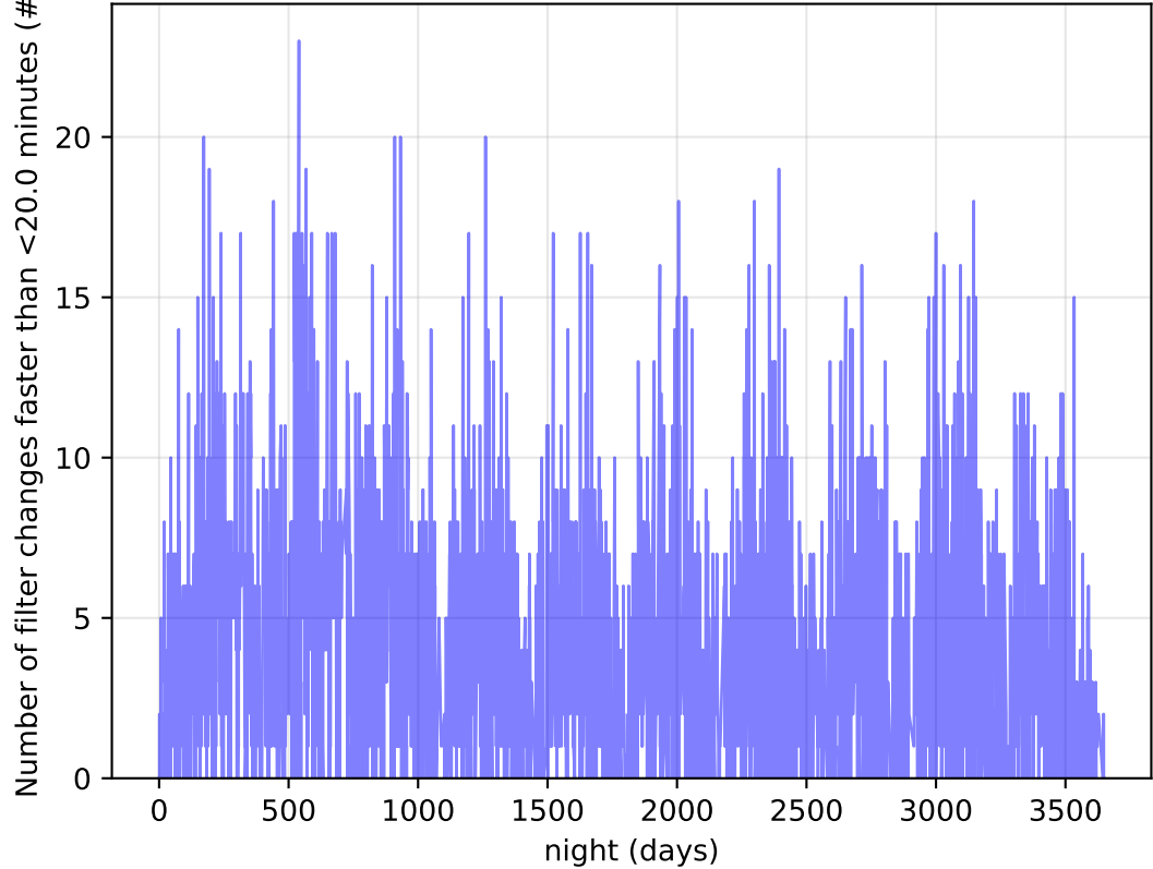
roll_pause_mjdp60_v3.4_10yrs Per Night: Number of filter changes faster than <20.0 minutes
