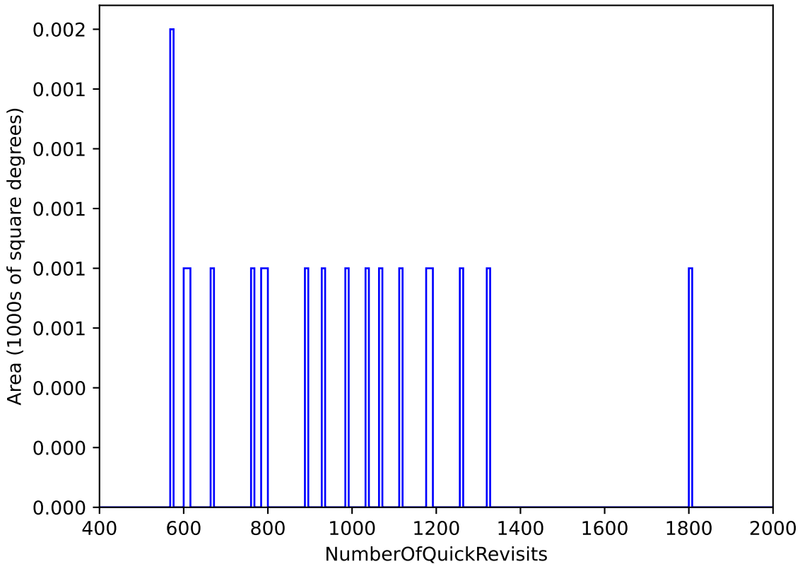
roll_pause_mjdp60_v3.4_10yrs WFD: NumberOfQuickRevisits
