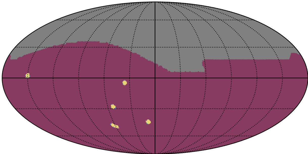
roll_pause_mjdp60_v3.4_10yrs All sky: NumberOfQuickRevisits
