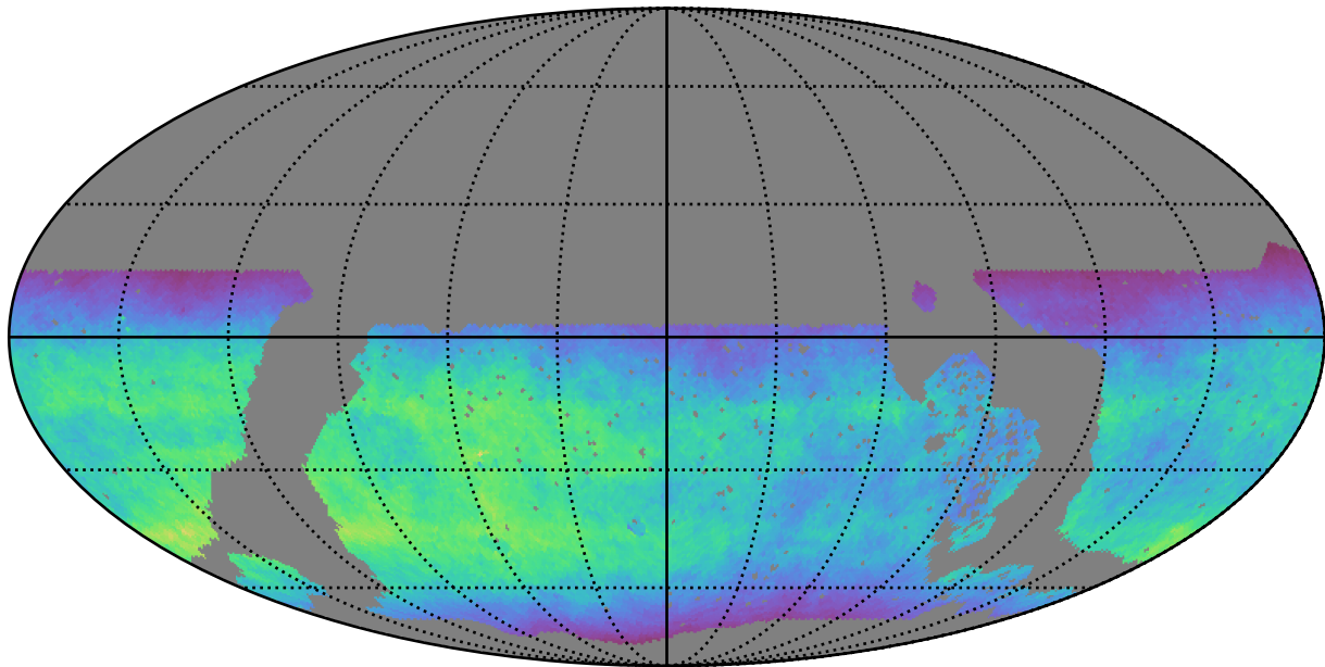
roll_pause_mjdp60_v3.4_10yrs WFD y band: Normalized Teff
