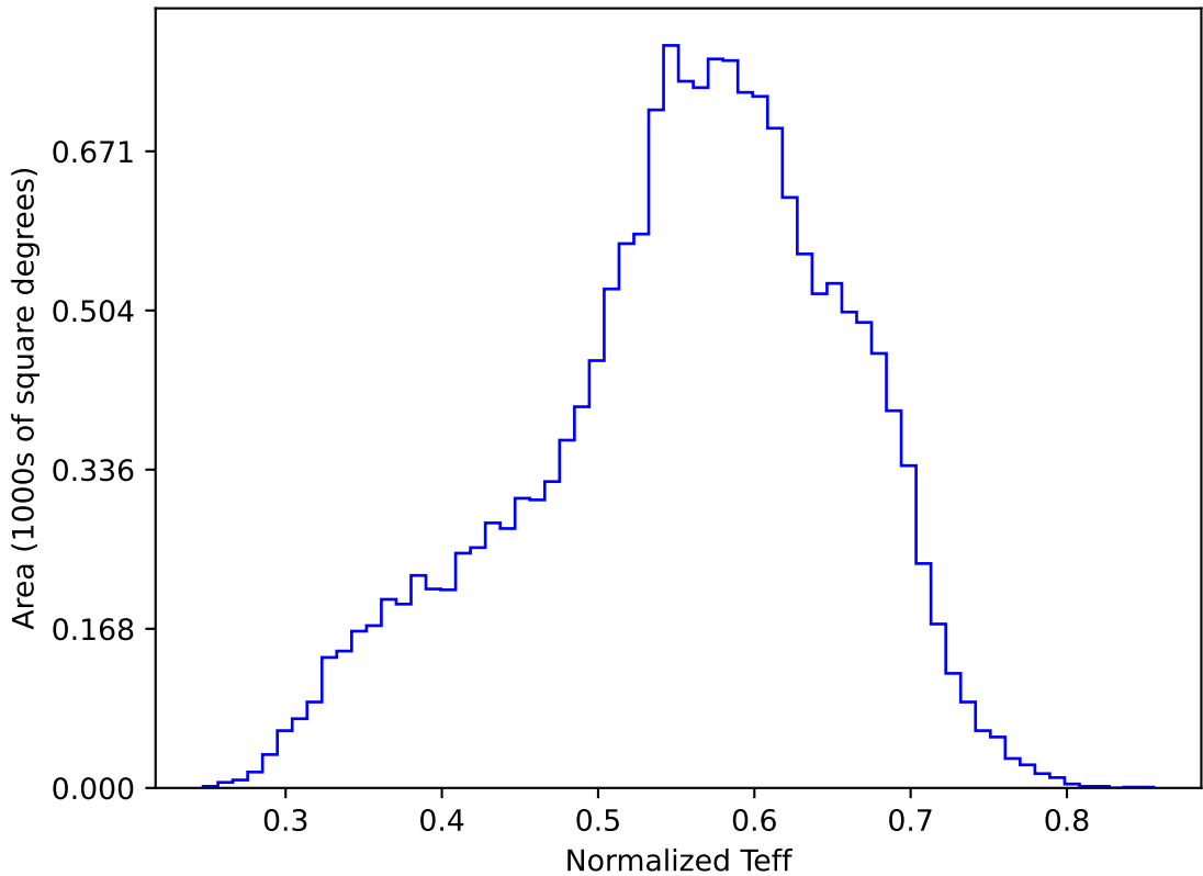
roll_pause_mjdp60_v3.4_10yrs WFD y band: Normalized Teff
