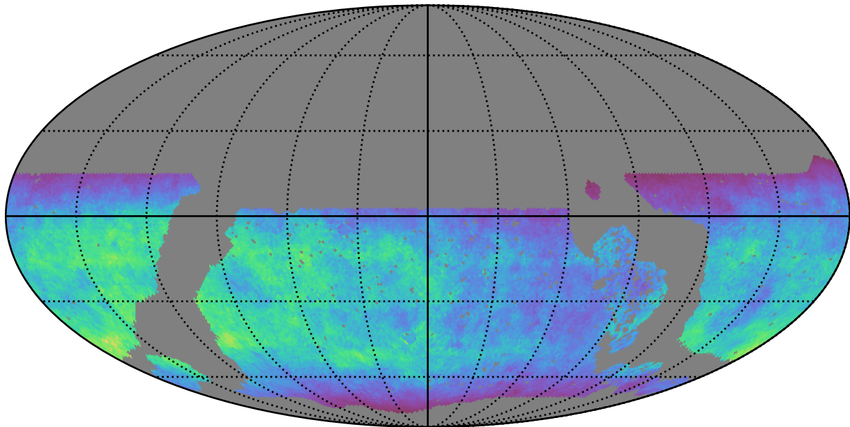
roll_pause_mjdp60_v3.4_10yrs WFD u band: Normalized Teff
