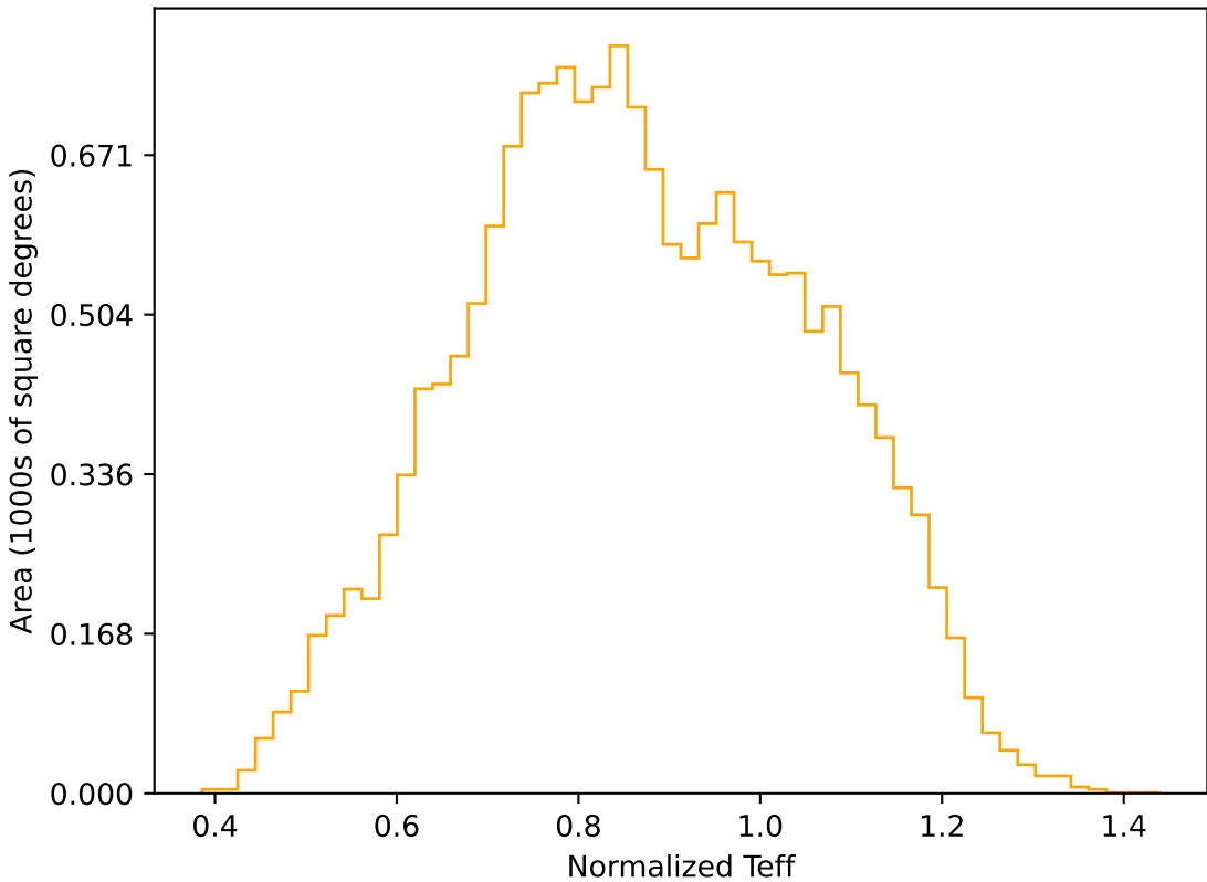
roll_pause_mjdp60_v3.4_10yrs WFD r band: Normalized Teff
