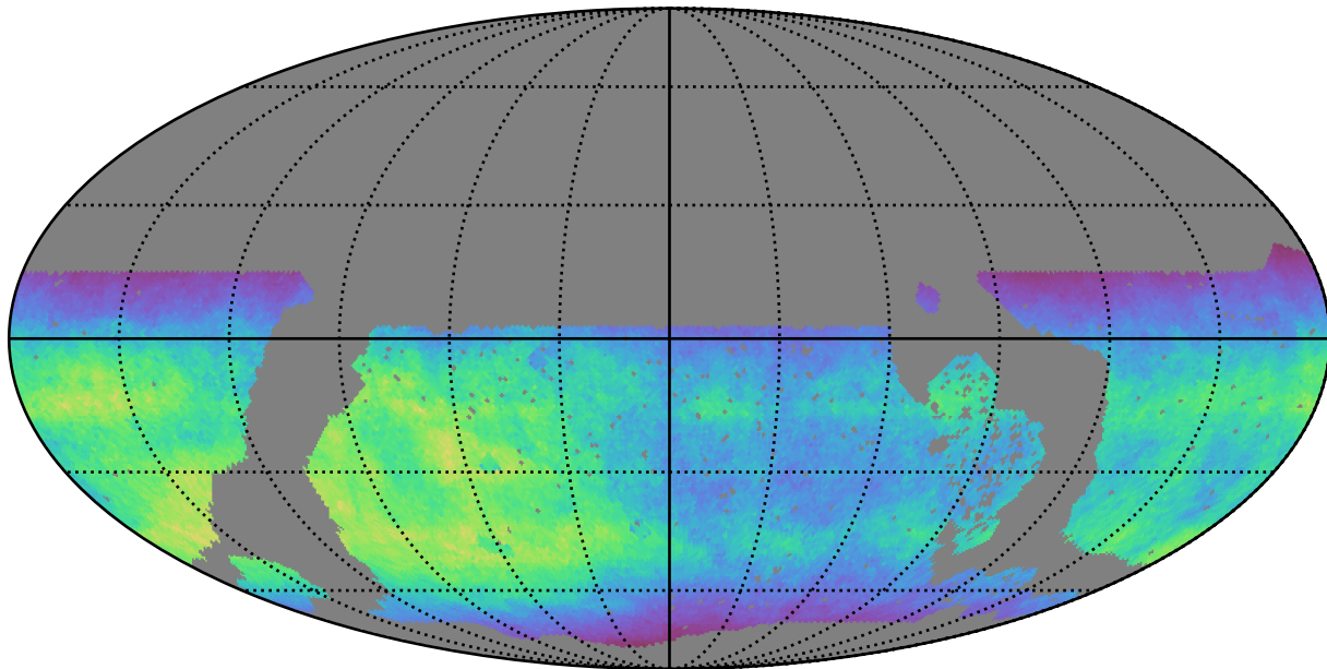
roll_pause_mjdp60_v3.4_10yrs WFD i band: Normalized Teff
