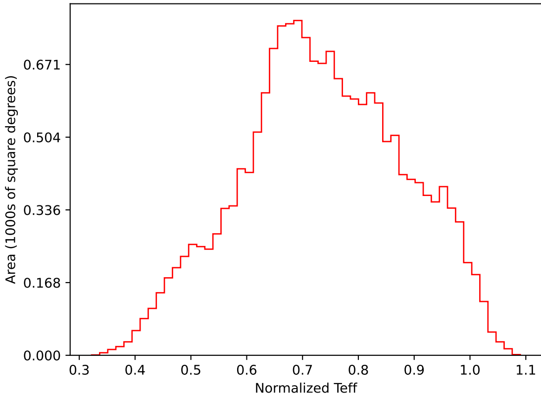
roll_pause_mjdp60_v3.4_10yrs WFD i band: Normalized Teff
