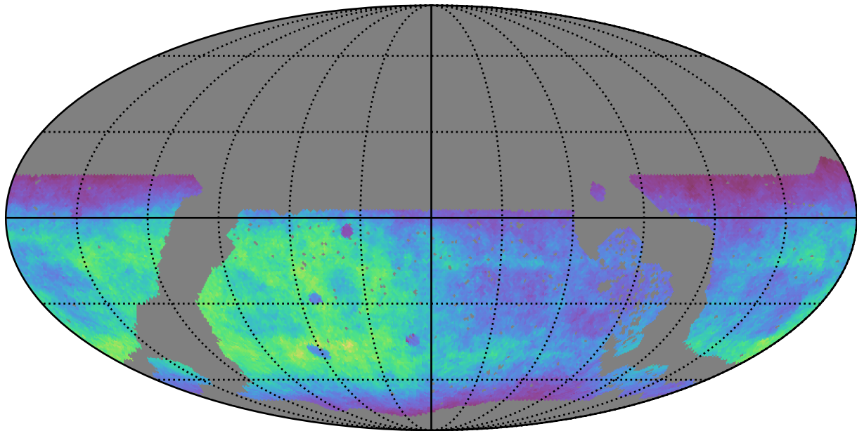
roll_pause_mjdp60_v3.4_10yrs WFD g band: Normalized Teff
