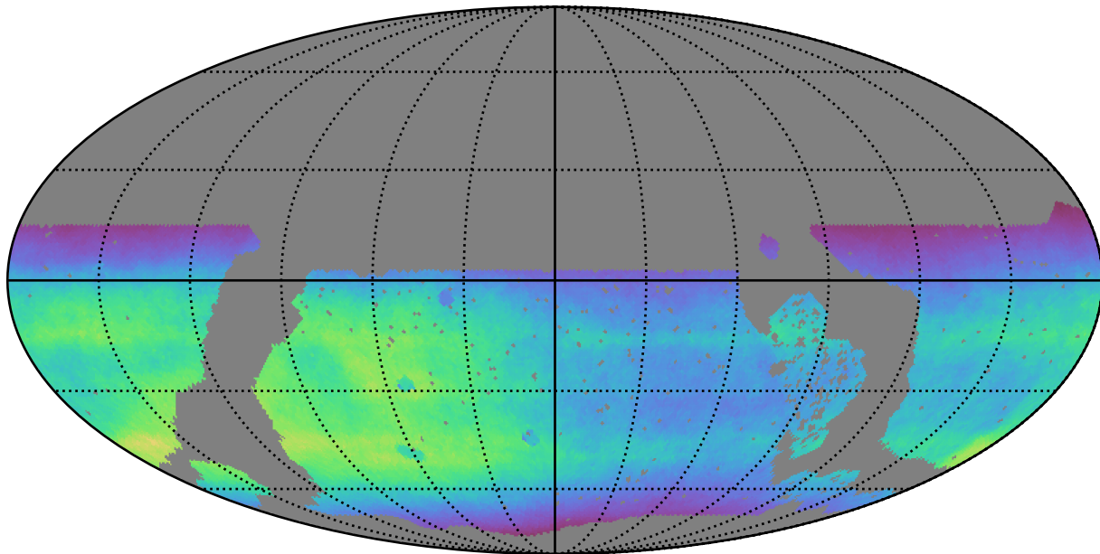
roll_pause_mjdp60_v3.4_10yrs WFD all bands: Normalized Teff
