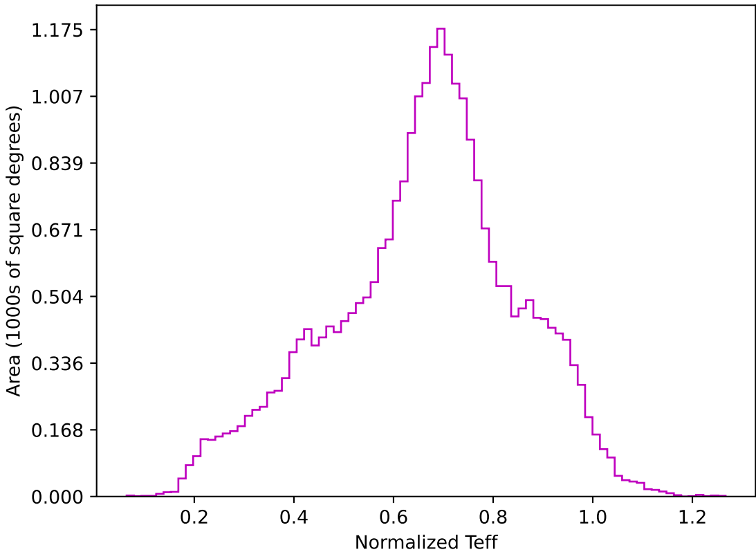
roll_pause_mjdp60_v3.4_10yrs All sky z band: Normalized Teff
