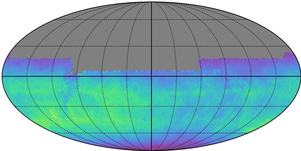
roll_pause_mjdp60_v3.4_10yrs All sky y band: Normalized Teff
