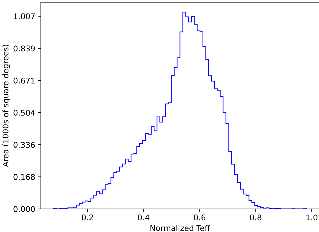
roll_pause_mjdp60_v3.4_10yrs All sky y band: Normalized Teff
