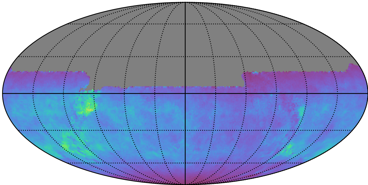
roll_pause_mjdp60_v3.4_10yrs All sky u band: Normalized Teff
