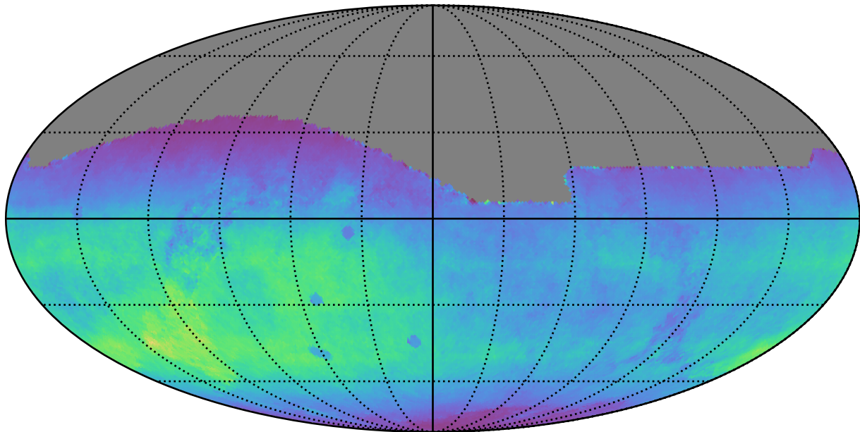
roll_pause_mjdp60_v3.4_10yrs All sky r band: Normalized Teff
