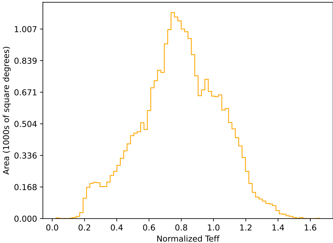
roll_pause_mjdp60_v3.4_10yrs All sky r band: Normalized Teff
