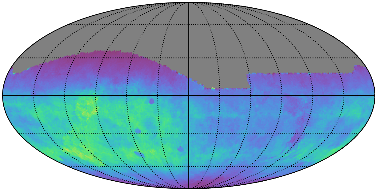
roll_pause_mjdp60_v3.4_10yrs All sky g band: Normalized Teff
