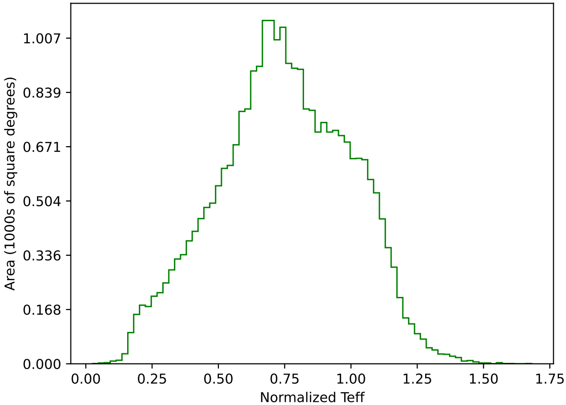
roll_pause_mjdp60_v3.4_10yrs All sky g band: Normalized Teff
