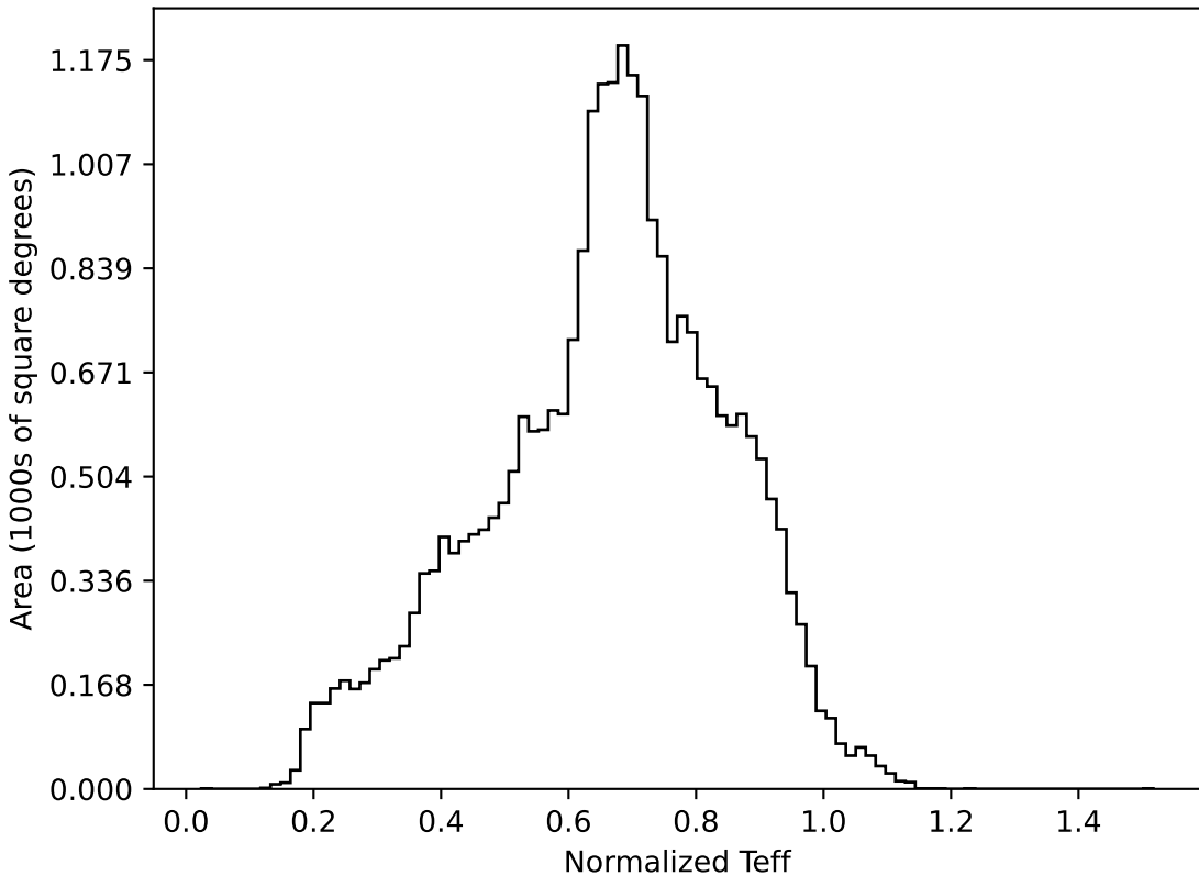
roll_pause_mjdp60_v3.4_10yrs All sky all bands: Normalized Teff
