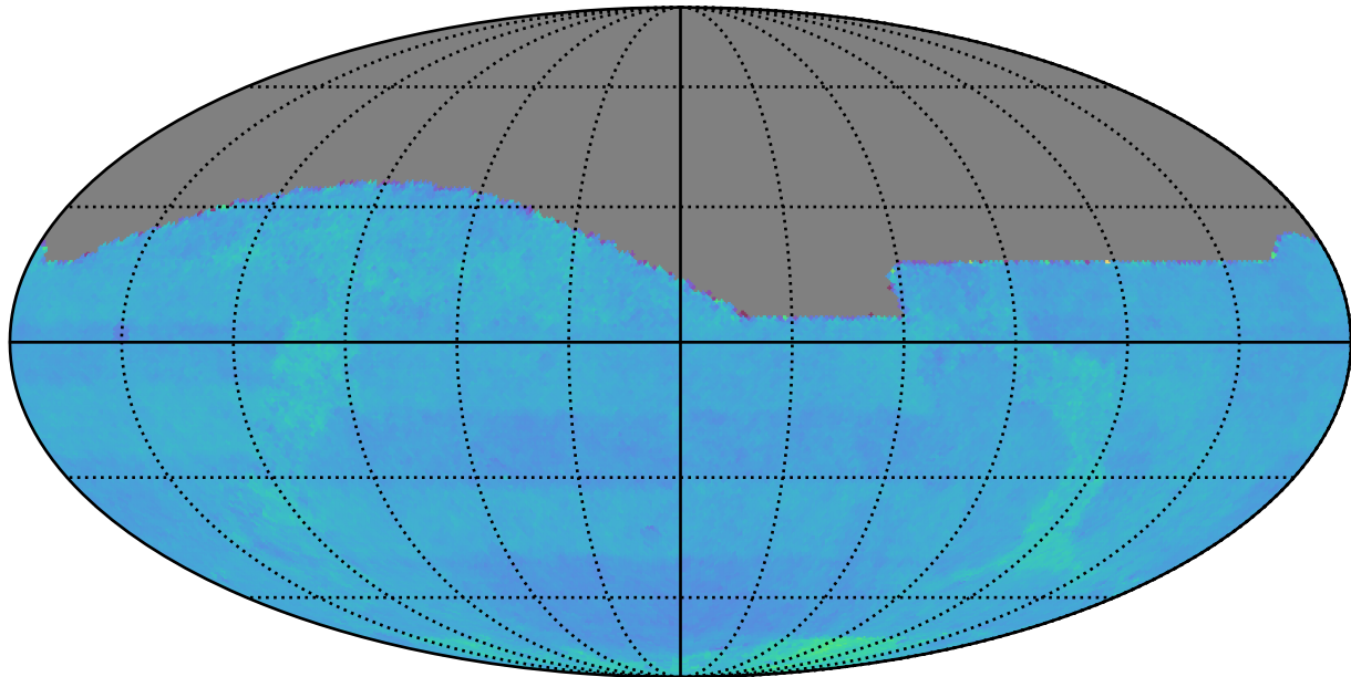
roll_pause_mjdp60_v3.4_10yrs All sky: Normalized Proper Motion Uncert @ 24.0
