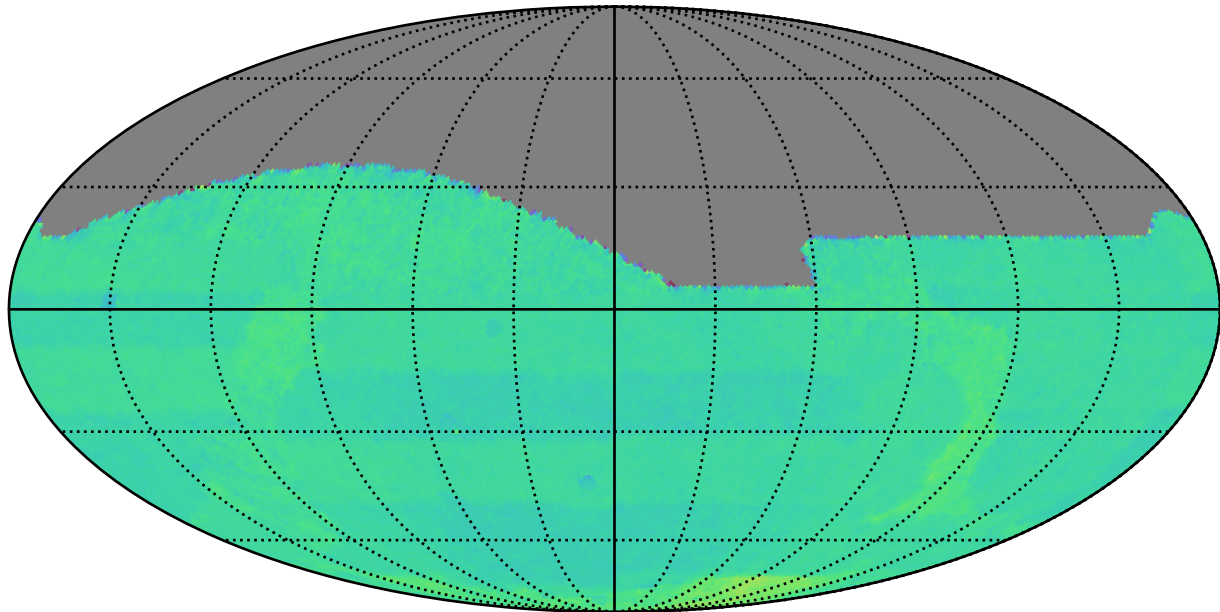
roll_pause_mjdp60_v3.4_10yrs All sky: Normalized Proper Motion Uncert @ 20.5
