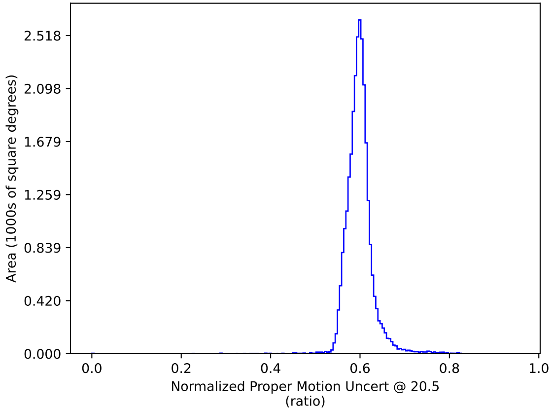
roll_pause_mjdp60_v3.4_10yrs All sky: Normalized Proper Motion Uncert @ 20.5
