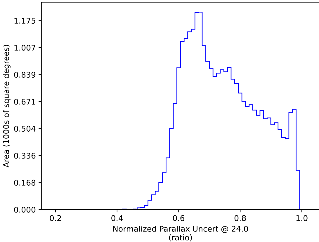
roll_pause_mjdp60_v3.4_10yrs All sky: Normalized Parallax Uncert @ 24.0
