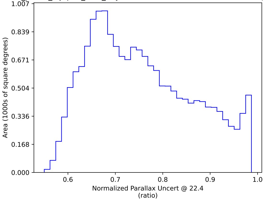
roll_pause_mjdp60_v3.4_10yrs WFD: Normalized Parallax Uncert @ 22.4
