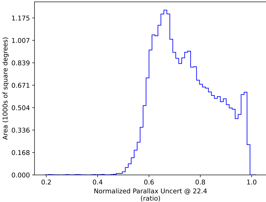
roll_pause_mjdp60_v3.4_10yrs All sky: Normalized Parallax Uncert @ 22.4
