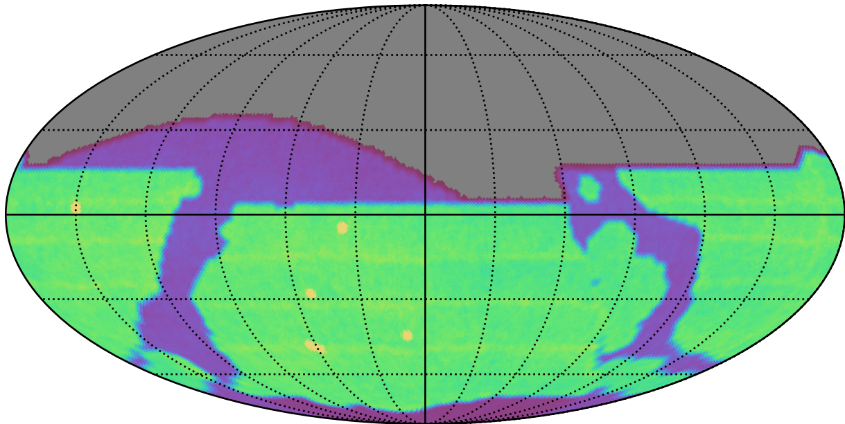
roll_pause_mjdp60_v3.4_10yrs All sky all bands: N Unique Nights
