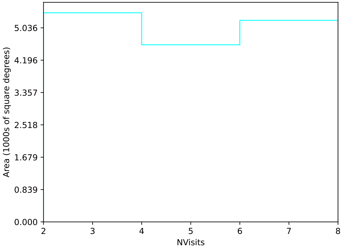
roll_pause_mjdp60_v3.4_10yrs Yr 3-4 u band: NVisits
