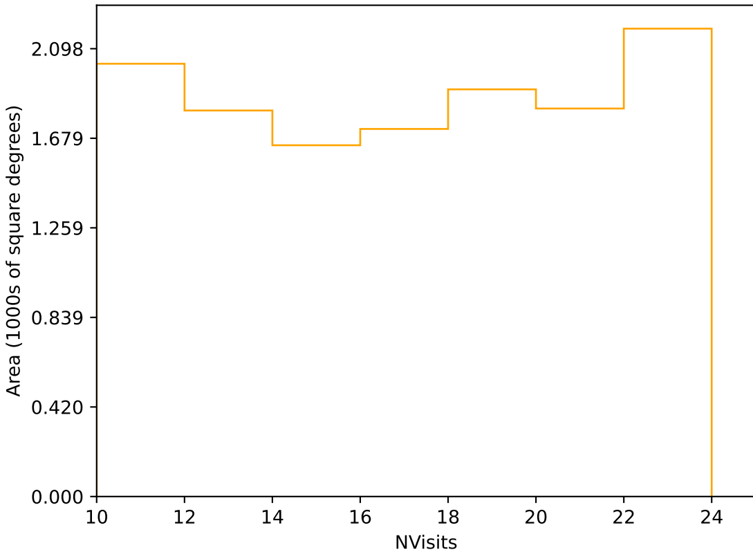
roll_pause_mjdp60_v3.4_10yrs Yr 3-4 r band: NVisits
