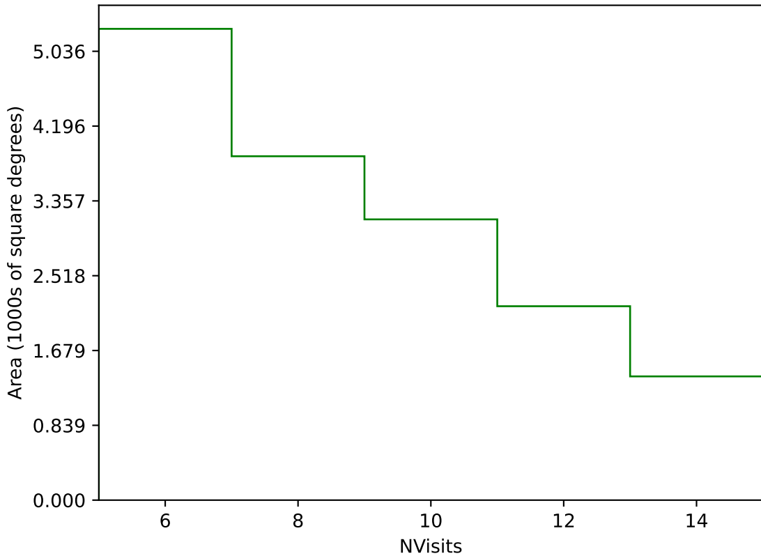
roll_pause_mjdp60_v3.4_10yrs Yr 3-4 g band: NVisits
