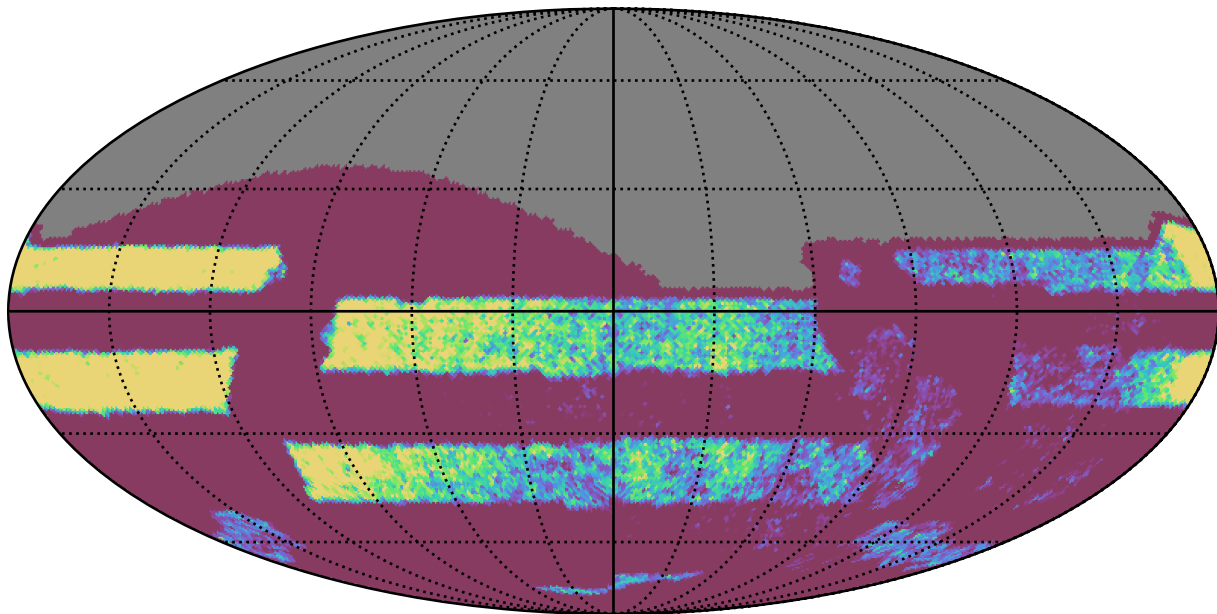
roll_pause_mjdp60_v3.4_10yrs Yr 3-4 all bands: NVisits
